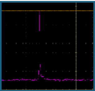
80 ps stable gain-switch pulse (Gain switch performance depends on laser diode)
